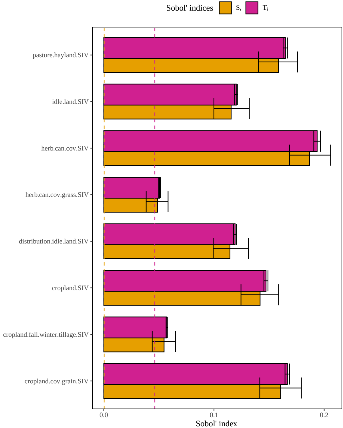
Figure 5. Results of a sensitivity analysis for the graypartridge model based on a geometric mean structure. Dashed lines represent baseline numerical approximation error for S_i and T_i ( i.e. , dummy variables).
